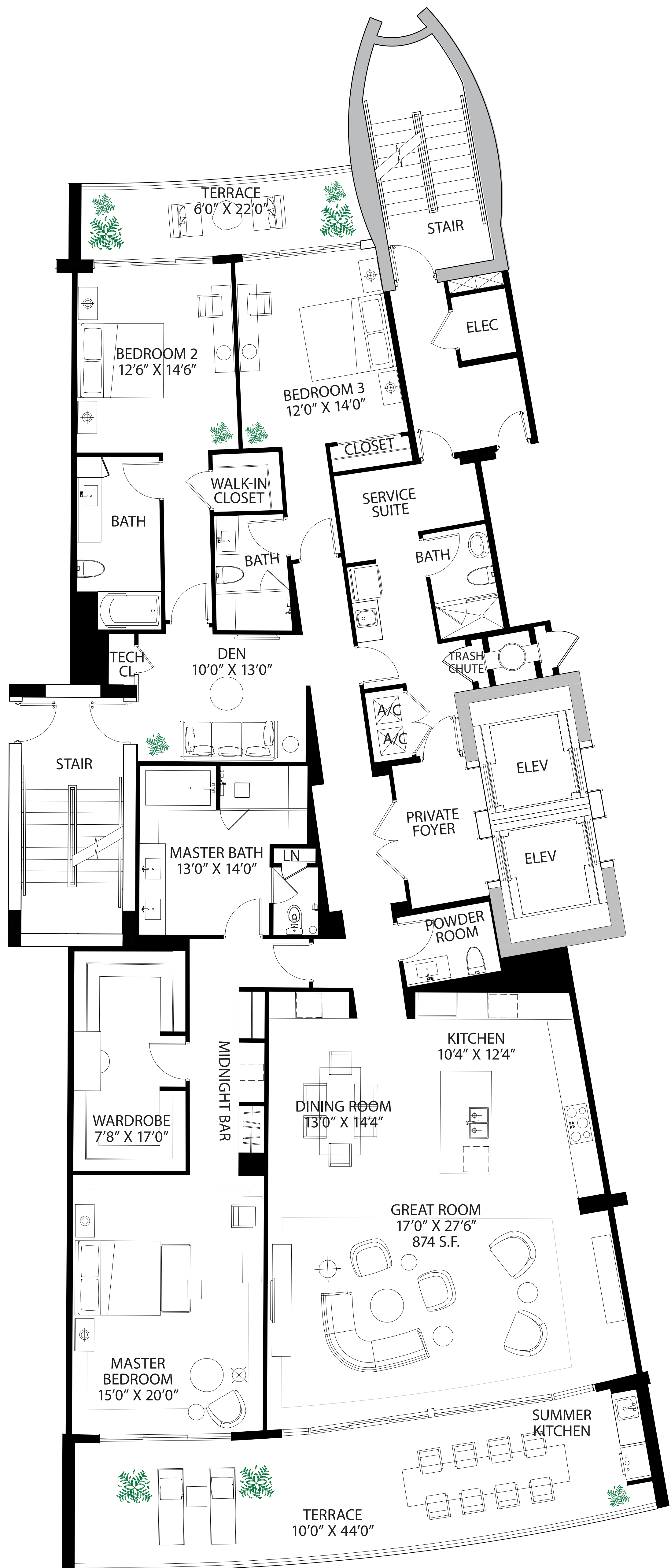
LOWER LEVEL
