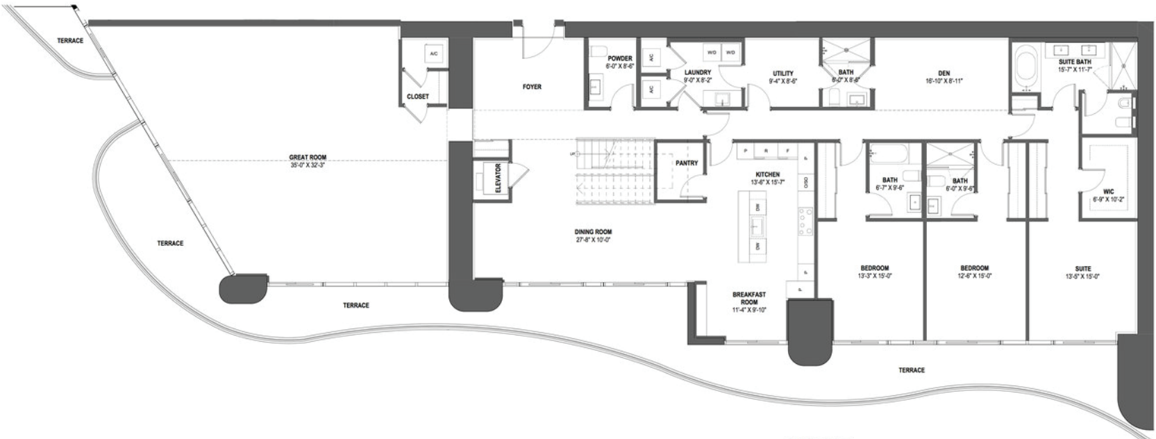
UNIT UPH-01 level 62 - floor plan 1/4" = 1'-0"
