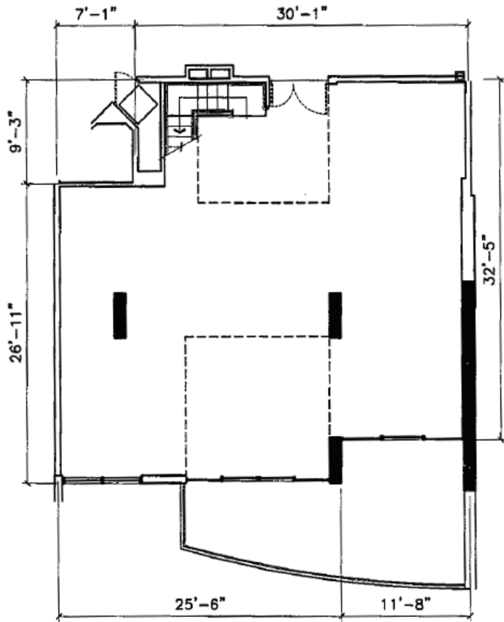
Lower Floor
